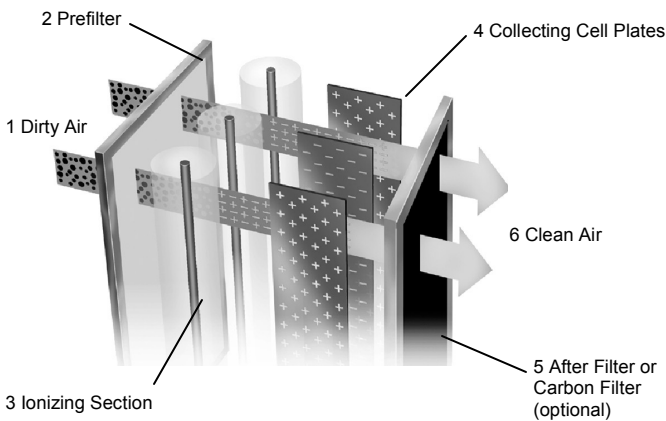
Electrostatic Precipitation
